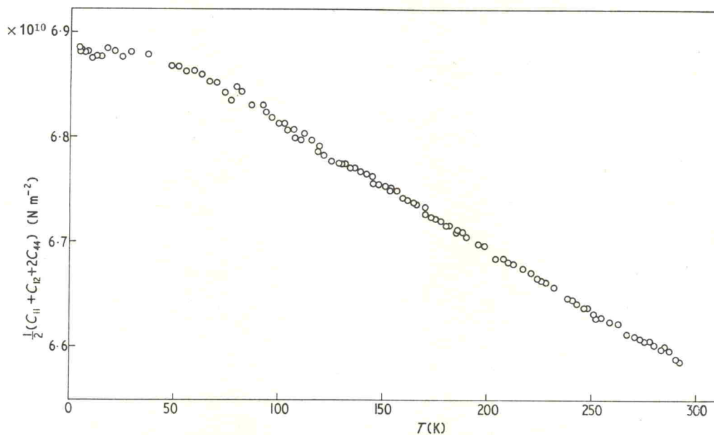
Figure 1. Variation of \frac{1}{2}(C_{11} + C_{12} + 2C_{44}) with temperature.
